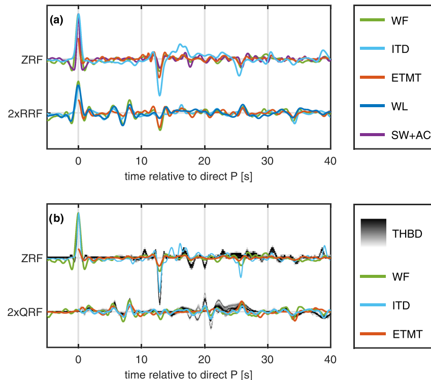
Figure 20. Comparison of P -to- S receiver functions derived by different methods. Note that horizontal components, that is, RRF and QRF, are upscaled by a factor of 2. (a) In the ZRT coordinate system. WF: Wiener filter deconvolution (green), ITD: iterative time domain deconvolution (light blue), ETMT: extended-time multitaper deconvolution (orange), WL: water-level deconvolution (blue, radial component only), SW+AC: spectral whitening and autocorrelation (purple, vertical component only). (b) In the LQT coordinate system. Gray shading is a data density plot of the THBD results, with darker shading indicating a more likely value. Abbreviations in the legend are the same as in (a).
