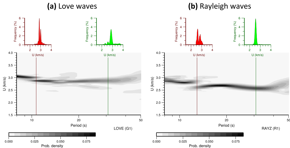
Figure 6. Dispersion analysis of the first wave trains of surface waves. The waveforms corresponding to (a) Love and (b) Rayleigh are band-pass filtered in 20 narrow band Gaussian filters between 8- and 50-s period. For each frequency, the envelope of the filtered signal is converted into a probability density function of group velocities and are plotted in gray scales. Two histograms (red for short periods and green for long periods, as indicated by the colored lines in the dispersion diagrams) are shown above the dispersion diagrams. For Love waves and vertical Rayleigh waves, the red histograms are shown for period values of 10.7 and 12.9 s, respectively. The green histograms corresponds to a period of 30.8 s.
