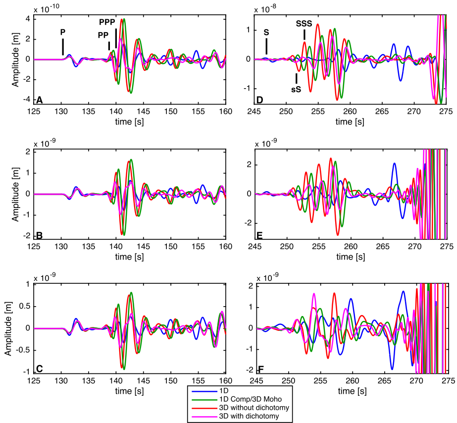
Fig. 14 Three-component ( A —Radial; B —Transverse; C —Vertical) synthetic seismograms computed at an epicentral distance of 16.2^\circ to the North-East of the event (inverted gray triangle in Fig. 12) using four different models. Model “1D” represents the one-dimensional model shown in Fig. 13E (black bold line); “1D/3D” (not shown) is a composite model consisting of a 1D crustal velocity component and a three-dimensional (3D) crustal thickness component; “3D” represent the three-dimensional models without (Fig. 13A–B) and with crustal dichotomy (Fig. 13C–D). A number of P-wave phases based on the “1D” model are indicated for reference. The mantle component underneath all models is assumed to be one-dimensional. Seismograms have been filtered between 2–100 s using a third-order Butterworth filter. The event is a double-couple ( M_w = 2.98 ) located at a depth of 3 km
