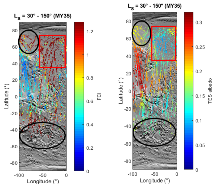
Figure 8. Left panel: LNO observations in MY35, from L_s = 30^{\circ} to 150^{\circ} . Colour points indicate the FCI values saturated at 3.5\sigma (see Section 4.1). Right panel: TES albedo values falling in each bin of the LNO tracks in MY35, from L_s = 30^{\circ} to 150^{\circ} . Red rectangle: correlation between high FCI values and region of low surface albedo. Black circle: example of high FCI values not correlated with regions of low surface albedo.
