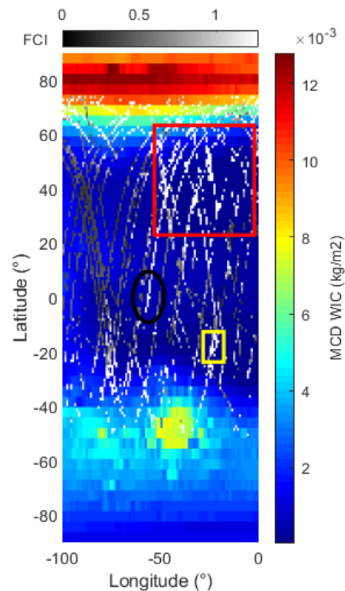
Figure 9. Comparison between the FCI results (grey scale) with the MCD Water Ice Column (colour scale) for all latitudes and longitude from 100°W to 0°. Grey scale: LNO observations in MY35, from Ls 30° to 150°. Saturated FCI values are in white ( >3.5\sigma , see Section 4.1). Colour scale: MCD Water ice column simulation for Ls 150° and 15 LTST.
