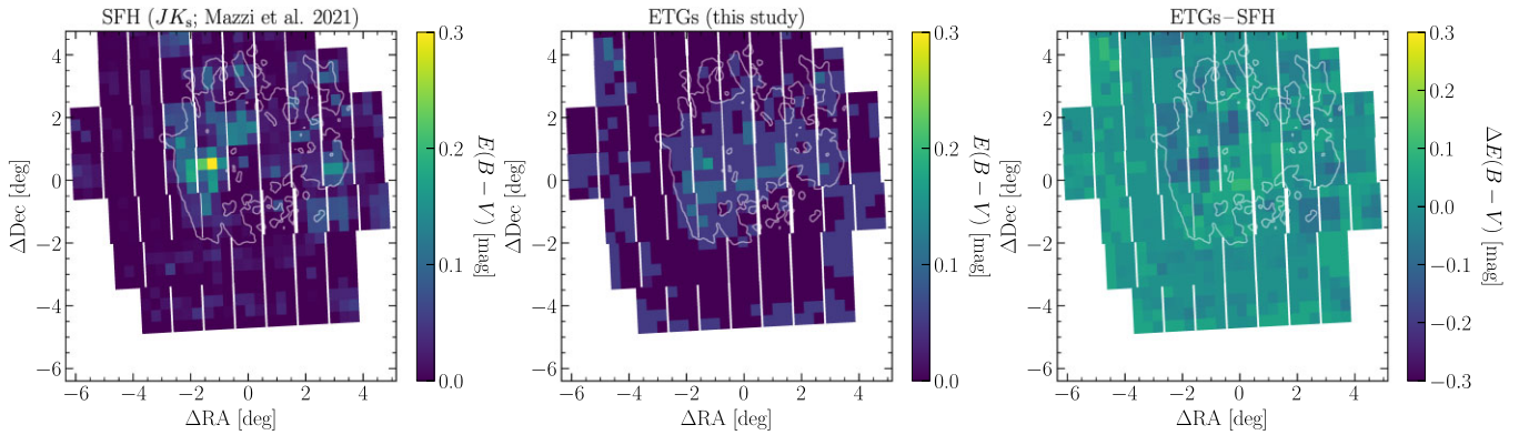
Figure 13. Left-hand panel: reddening map of the LMC derived from the SFH study by Mazzi et al. (2021). The spatial resolution corresponds to bins of 21.0 \times 21.5 arcmin 2 whereas the area shown is the same as in Figs 8, 9, and 11, hence the white space in the south and not all bins shown in the north. The contour represents the low-level pervasive dust associated with the central regions of the LMC as traced by the IRAS 100- \mu m emission. Note that the colour bar range has been limited to 0 \leq E(B - V) \leq 0.3 mag to better illustrate low-level features within the maps. Middle panel: as the left-hand panel, but showing the ETG reddening map adopting the spatial resolution of Mazzi et al. Right-hand panel: as the left-hand panel, but showing the differential reddening map, such that \Delta E(B - V) = E(B - V)_{\text{ETG}} - E(B - V)_{\text{SFH}} . Note that the colour bar range has been limited to -0.3 \leq E(B - V) \leq 0.3 mag to better illustrate low-level features within the map.
