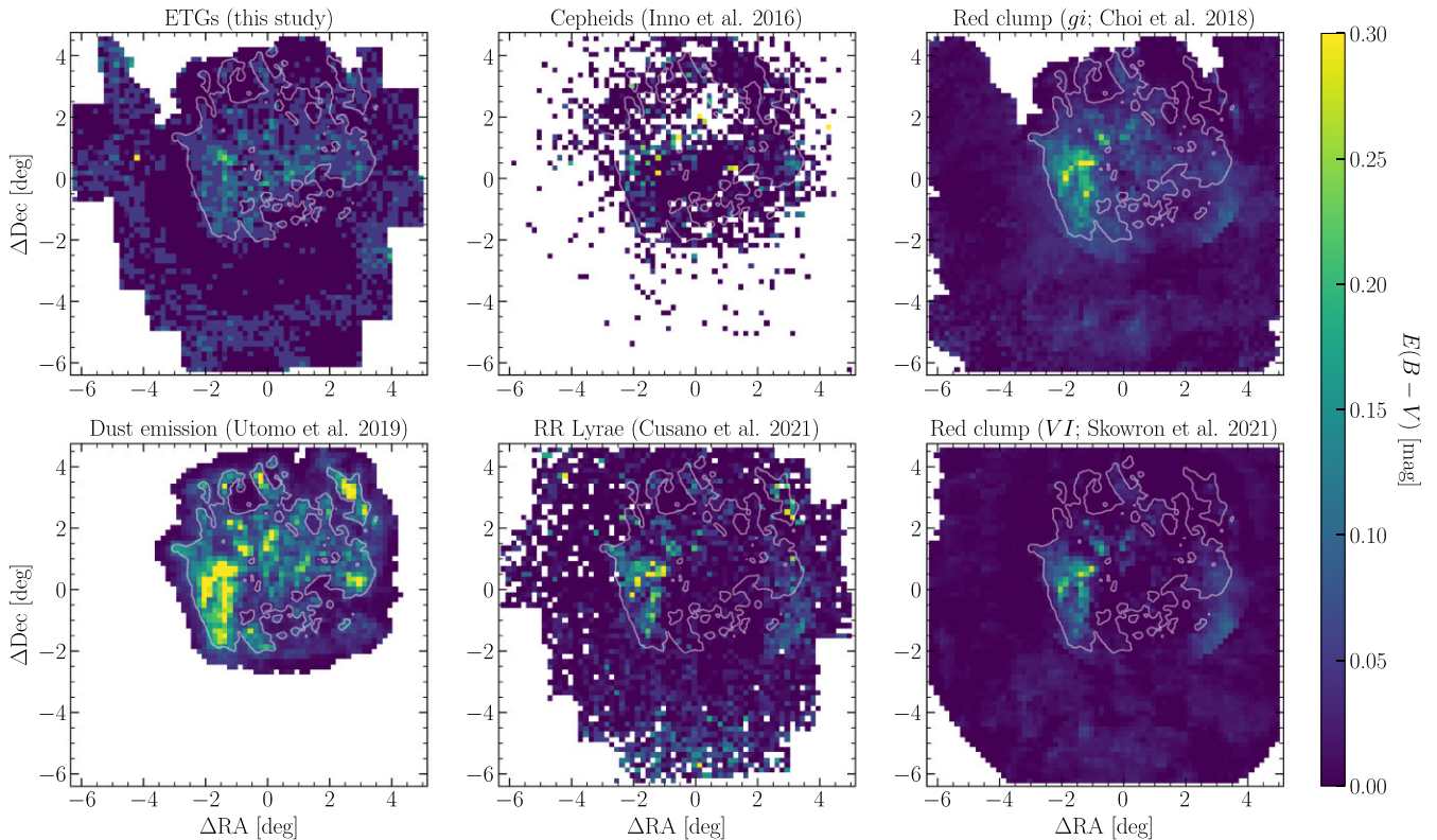
Figure 11. 10 \times 10 \text{ arcmin}^2 resolution reddening maps of the LMC. Each panel refers to a different literature source/tracer. The contour in each panel represents the low-level pervasive dust associated with the central regions of the LMC as traced by the IRAS 100\text{-}\mu\text{m} emission. Note that the colour bar range has been limited to 0 \leq E(B - V) \leq 0.3 mag to better illustrate low-level features within the maps. Note also that the ETG extinctions should be roughly twice that of the Cepheids, RR Lyrae, and RC values since the latter do not sample the full path through the LMC.
