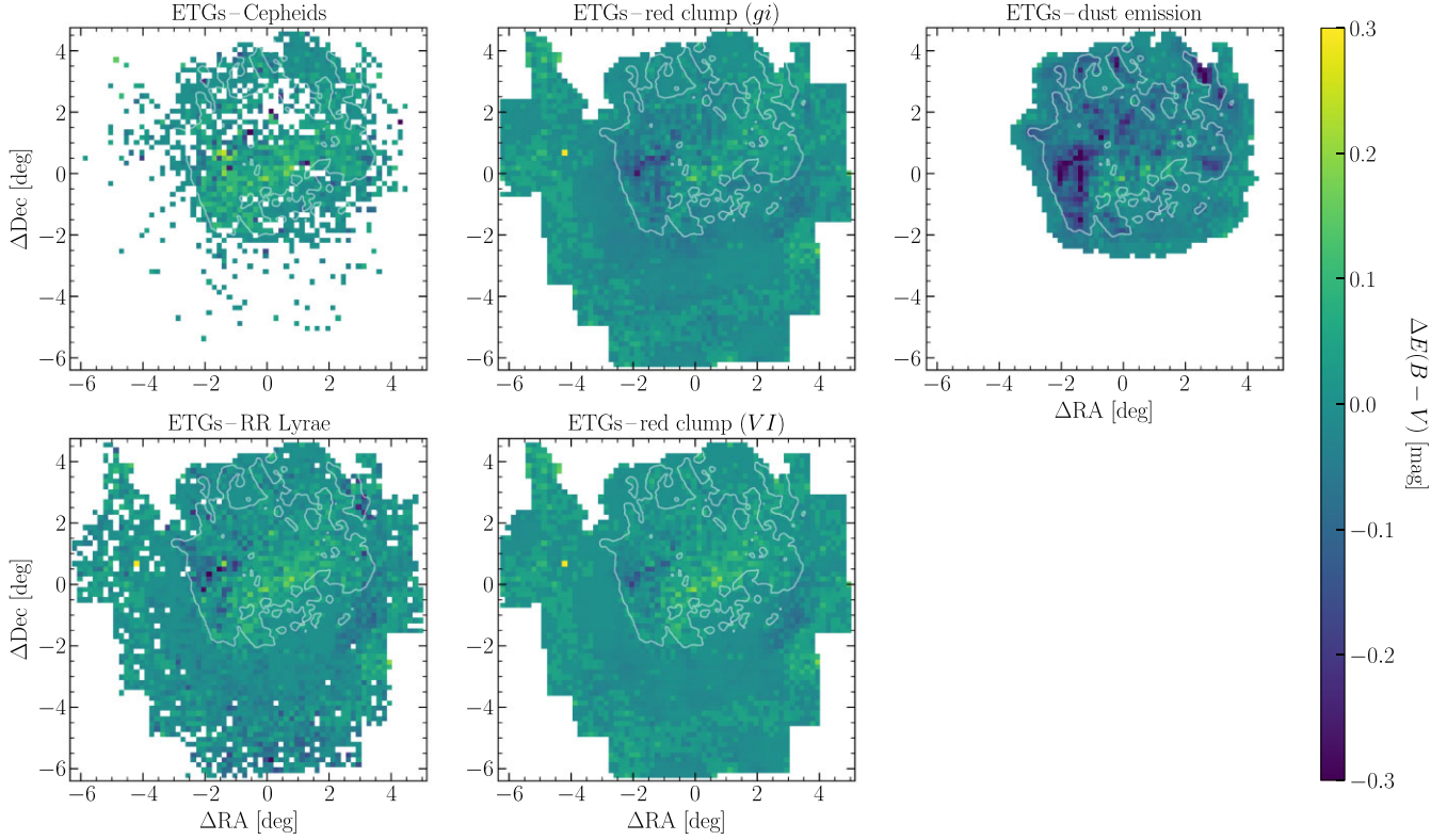
Figure 12. As Fig. 11, but showing a 10 \times 10 arcmin 2 resolution differential reddening maps of the LMC, such that \Delta E(B - V) = E(B - V)_{\text{ETG}} - E(B - V)_{\text{tracer}} . Note that the colour bar range has been limited to -0.3 \leq E(B - V) \leq 0.3 mag to better illustrate low-level features within the maps.
